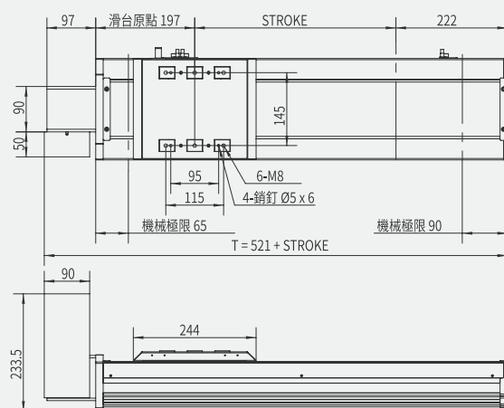
AIMTW202-4P-LF-PF 馬達右側間接安裝 motor rightside parallel installed
