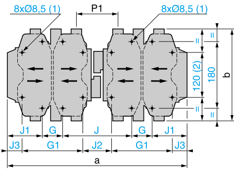
2 x LC1D410, D475, D620
