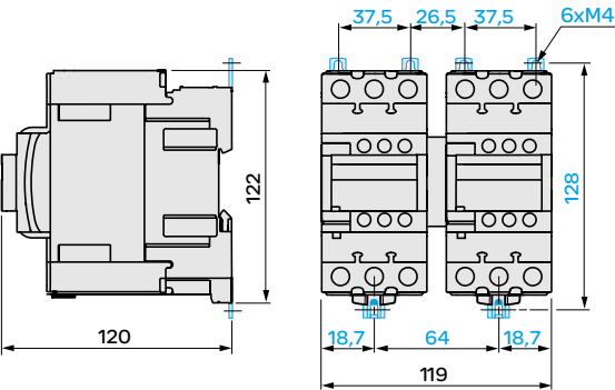
2 x LC1D40A 至 D65A
